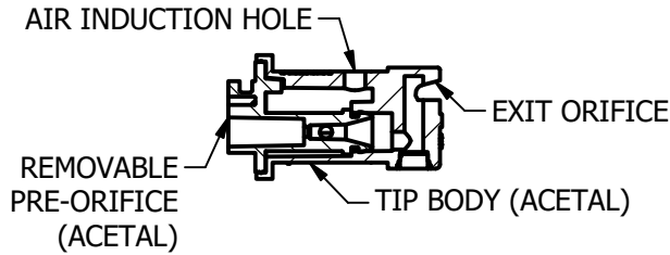
TTI110_-VP SPRAY TIP (CROSS SECTION VIEW)
