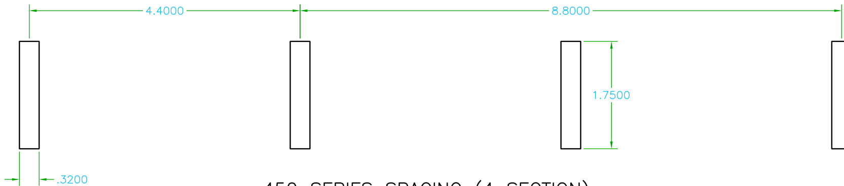
450 SERIES SPACING (4 SECTION)
