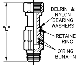
CROSS - SECTION VIEW (TYPICAL)
