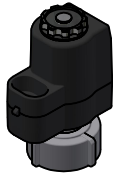
TEEJET DIAPHRAGM CHEMSAVER PART NO. 58577 DIAPHRAGM: CP56709-VI
