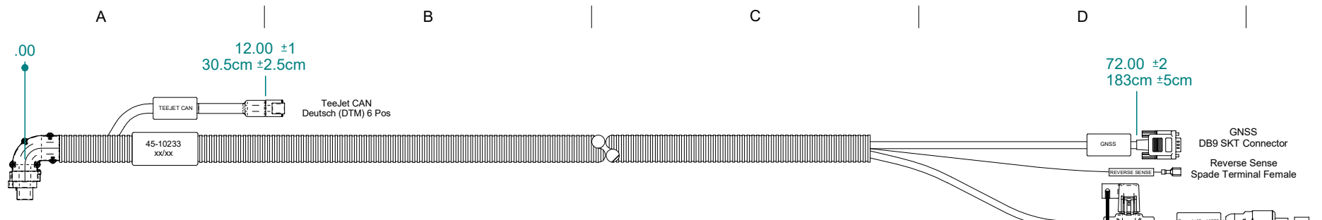
AMP SuperSeal Connector 34 Pos. w/ Skts
