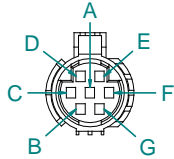
Metri-Pack Shroud 7 Pos. w/Pins
