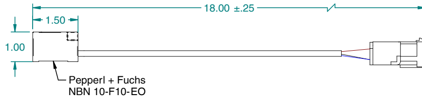
Weather-Pack 4 Pos. Shroud STKD w/Pins
