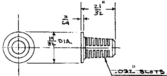
# 4514 SLOTTED STRAINER (BRASS)
