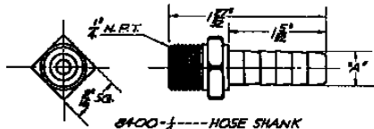
8400-1/4---HOSE SHANK
