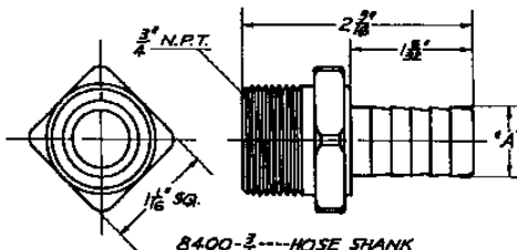
8400-3/4---HOSE SHANK
