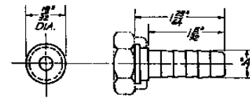
8400---HOSE SHANK
