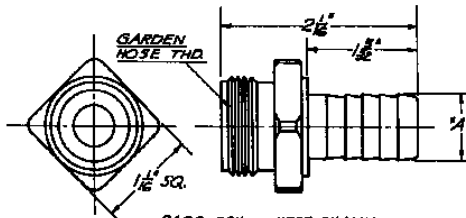
8400-6GH---HOSE SHANK
