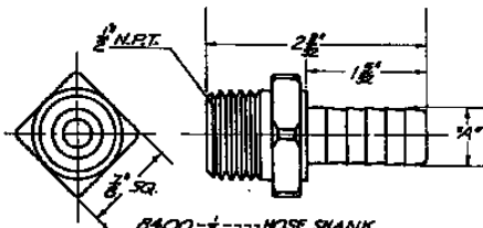
8400-1/2---HOSE SHANK
