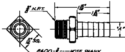
8400-3/8---HOSE SHANK
