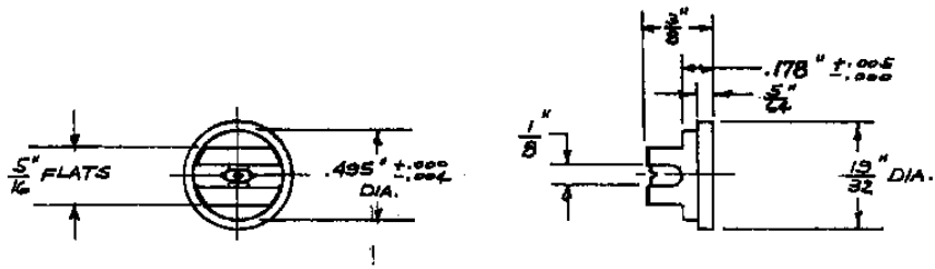
--- 017 TO --- 08 FLAT ATOMIZING SPRAY TIPS
