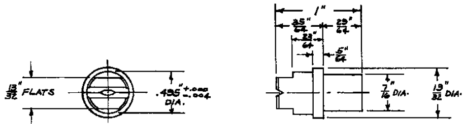
--- 30 & --- 40 FLAT ATOMIZING SPRAY TIPS
