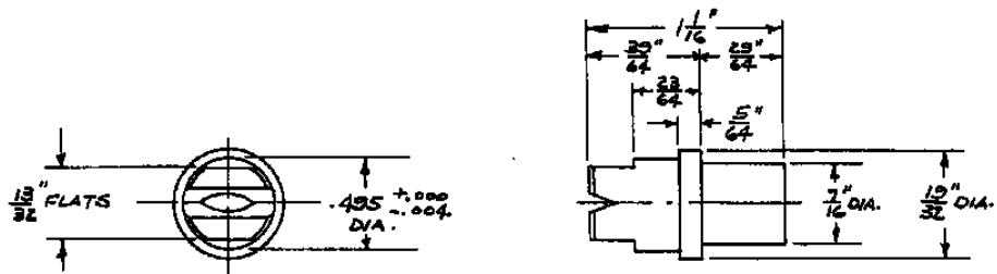
--- 50 TO --- 70 FLAT ATOMIZING SPRAY TIPS
