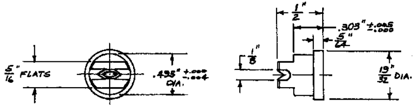
--- 10 & --- 20 FLAT ATOMIZING SPRAY TIPS
