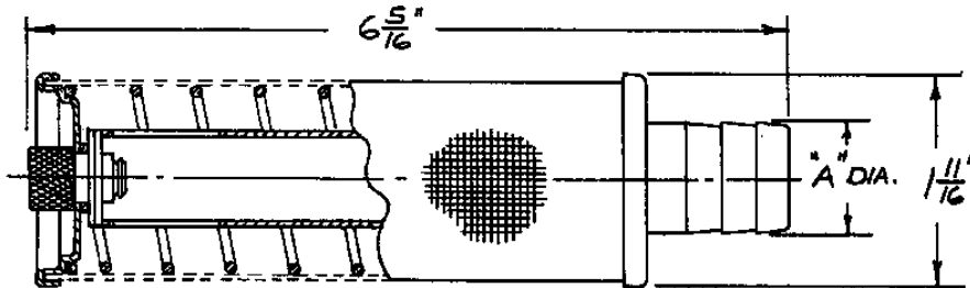
NO. 7130-1050AL SUCTION STRAINER
