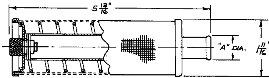
NO. 7130-675 & NO. 7130-800 SUCTION STRAINERS
