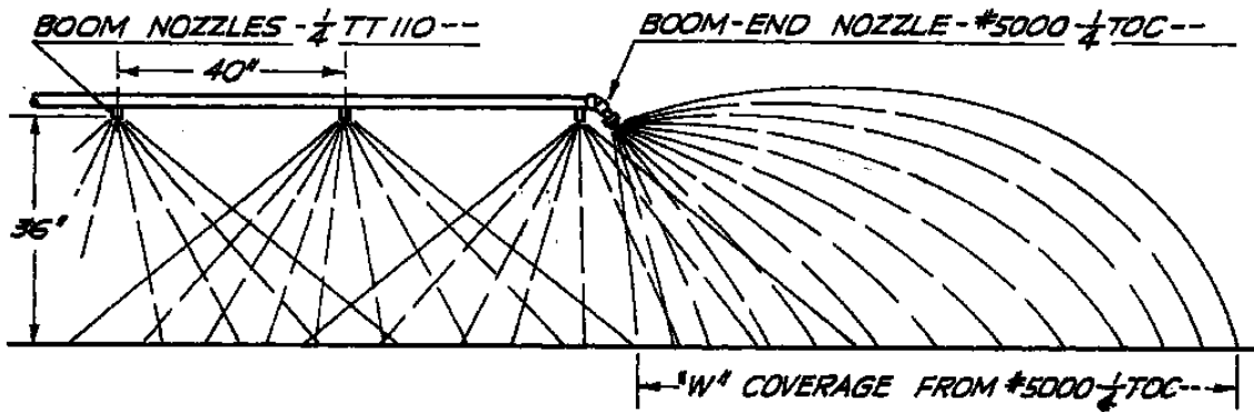
TABULATION BASED ON SPRAYING WATER AT 70°F. TEMPERATURE
