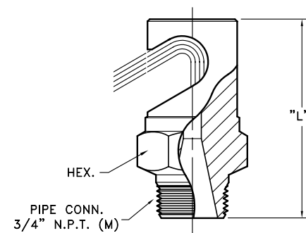
3/4KLC-- NOZZLES ARE AVAILABLE IN BRASS AND STAINLESS STEEL.
