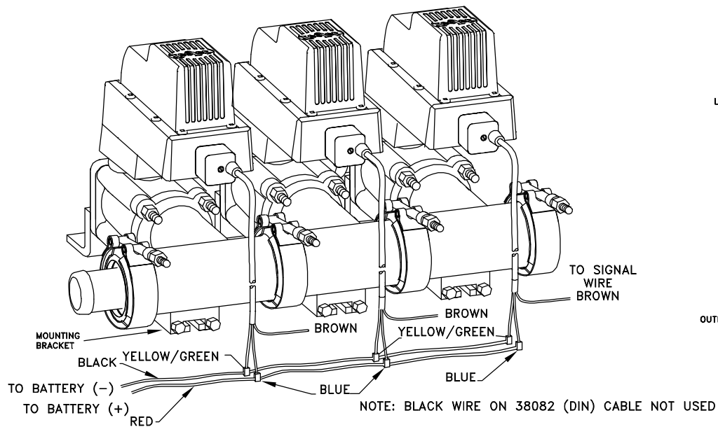
WIRING DIAGRAM (POSITIVELY SWITCHED)
