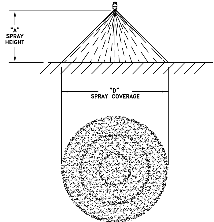
TYPICAL SPRAY PATTERN
