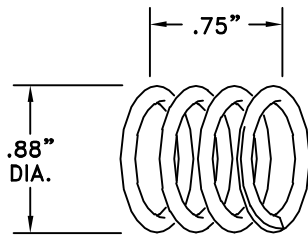
CP15167-302SS SPRING TYPE 302 STAINLESS STEEL (1 REQ'D)
