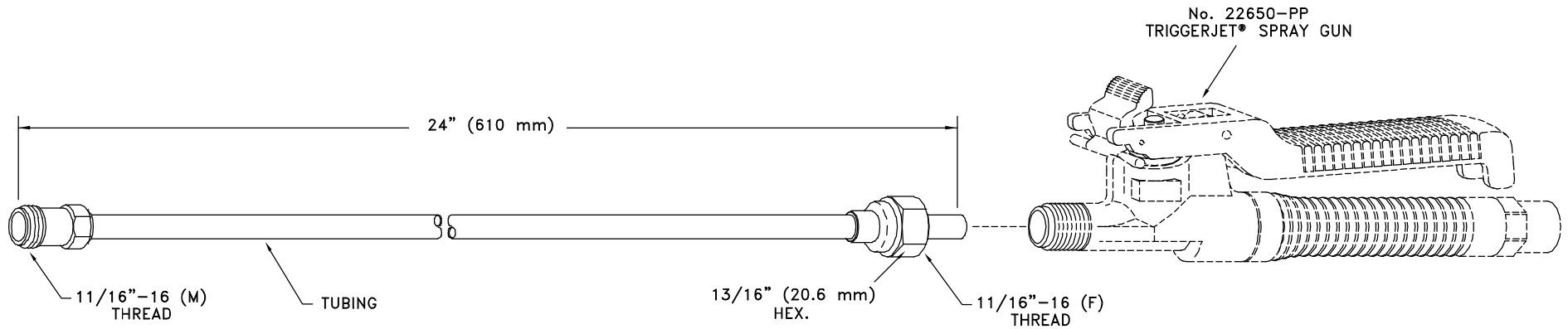
No. 38166-7715-24 EXTENSION ASSEMBLY
