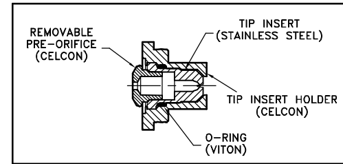
DG----VS SPRAY TIP (CROSS SECTION VIEW)
