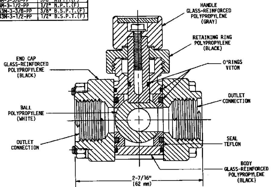
CROSS SECTION SIDE VIEW
