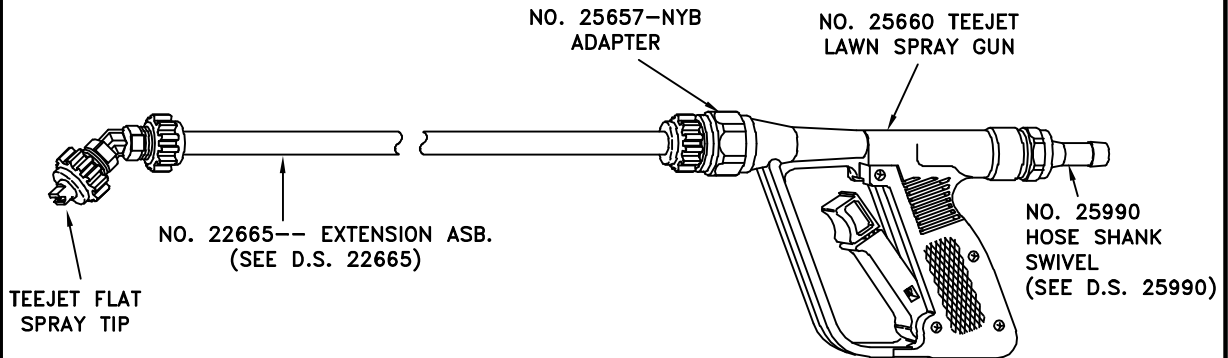
LOW VOLUME SPRAY GUN ASSEMBLY
