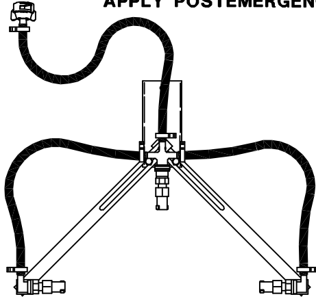
MODEL NO. 23770-SS ROW APPLICATION KIT (Supplied without spray tips and strainers)
