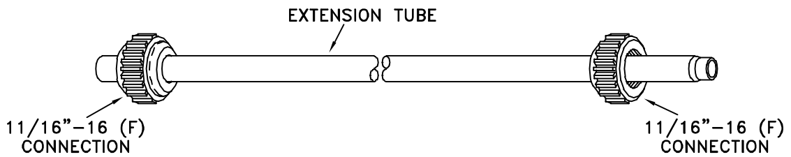
No. 22665-- EXTENSION ASSEMBLY
