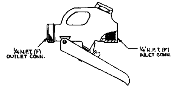
NO. 7900 TRIGGER VALVE WITH SHORT NON-LOCKING TRIGGER
