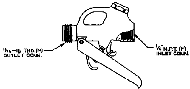
NO. 4688 TRIGGER VALVE
