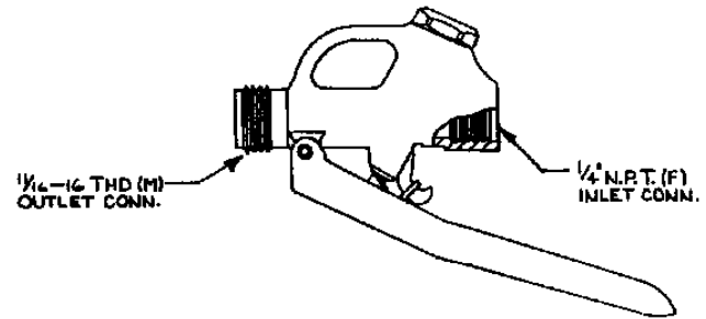
NO. 6446 TRIGGER VALVE WITH LONG NON-LOCKING TRIGGER
