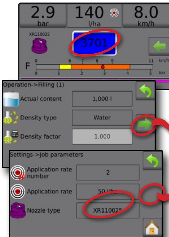
Figure 53: Tank filling
