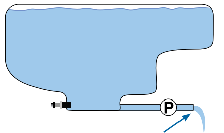
Figure 38: Tank shape calibration
