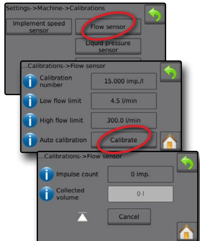
Figure 22: Flow sensor
