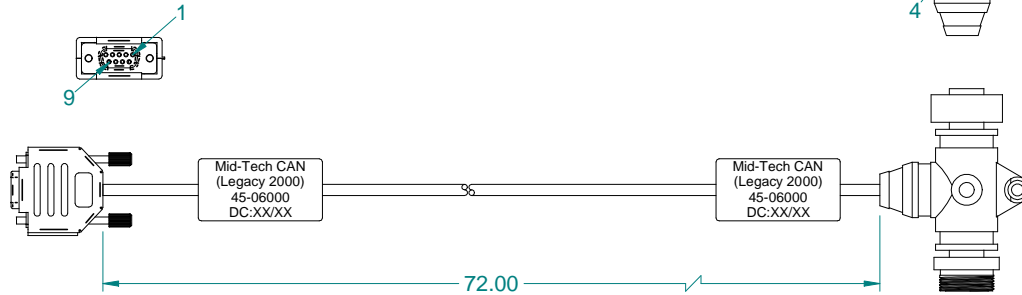
Connector DB9 Female Skt Pin Out
