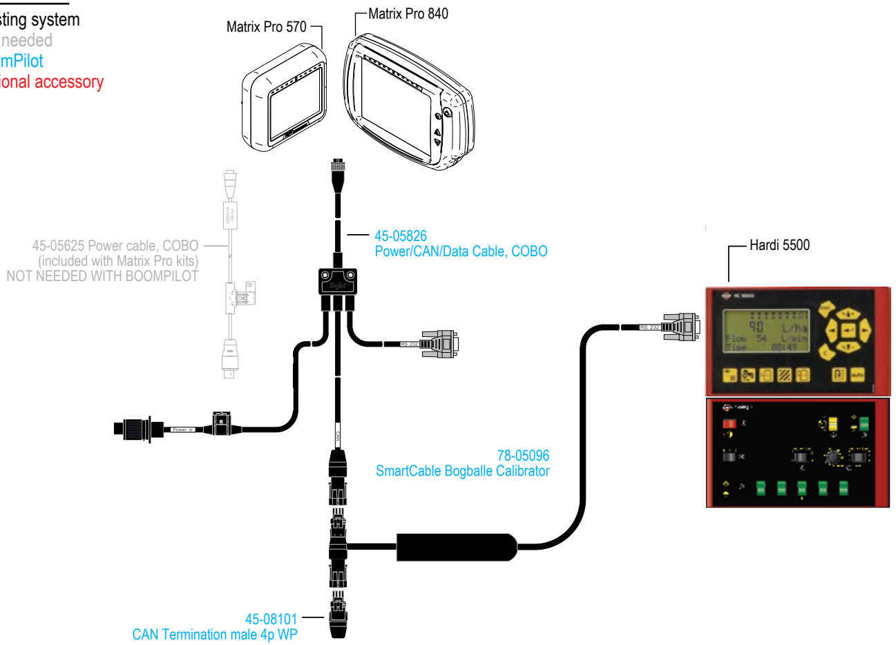
Figure 1: System diagram
