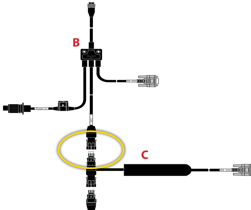
Figure 4: Connect power/CAN/data cable to SmartCable
