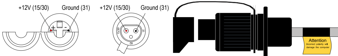
Figure 5: COBO Cable
